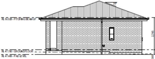
FRONT ELEVATION (SOUTH-WEST) SCALE: 1:100
