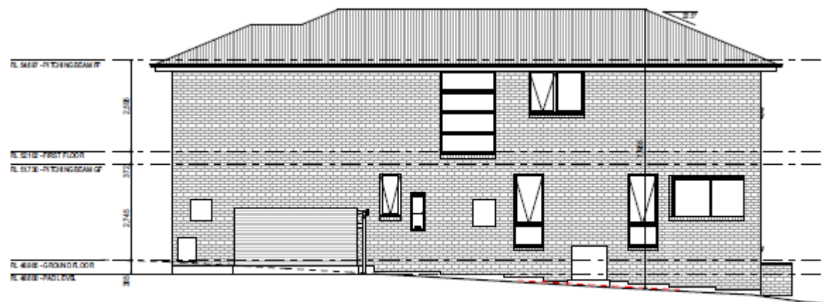
RIGHT ELEVATION (SOUTH-EAST) SCALE: 1:100
