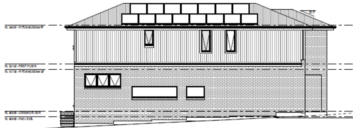
LEFT ELEVATION (NORTH-WEST) SCALE: 1:100
